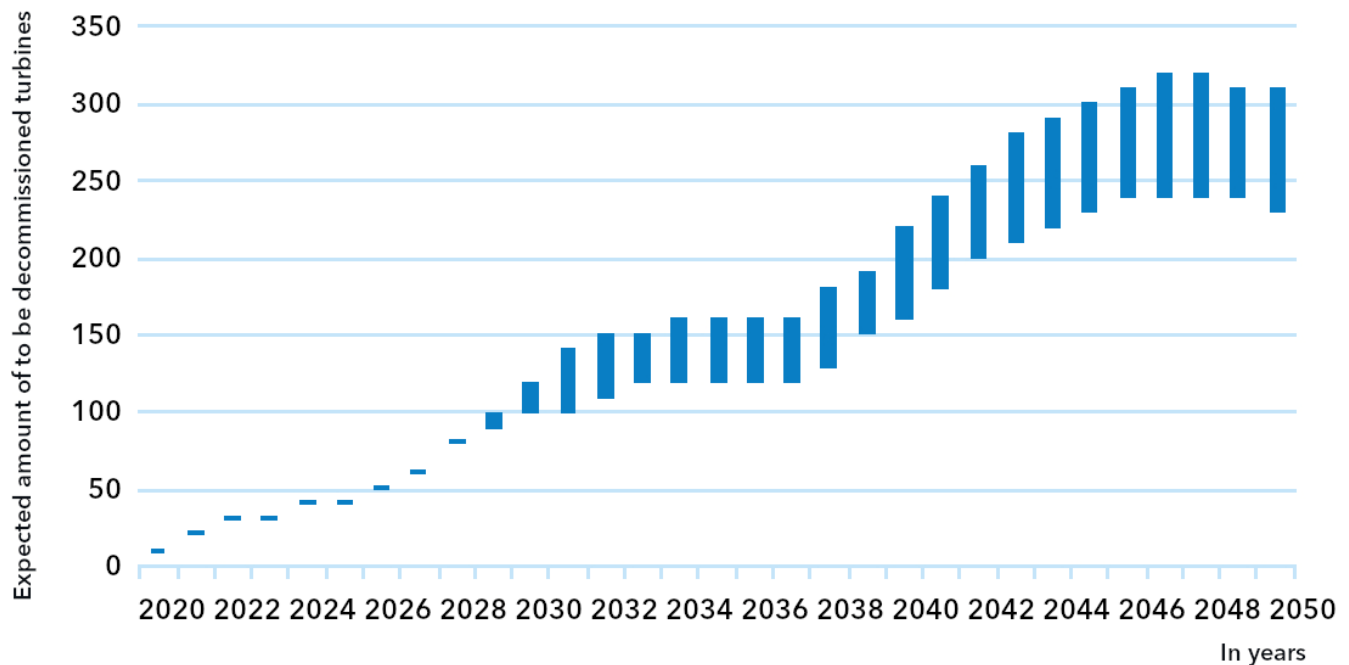
Figure 2: The residual flow of the expected amount of offshore wind turbines in the southern North Sea area (Hajonides et al., 2020) 6
