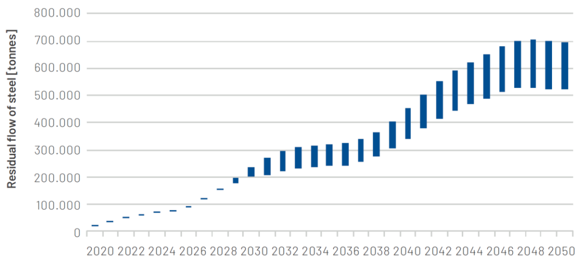
Figure 21: Residual flow of steel [tonnes] resulting from offshore wind farm decommissioning in the southern North Sea (Hajonides et al., 2020).
