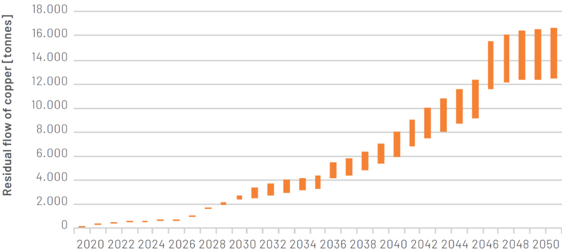
Figure 23: Residual flow of copper [tonnes] resulting from offshore wind farm decommissioning in the southern North Sea (Hajonides et al., 2020).
