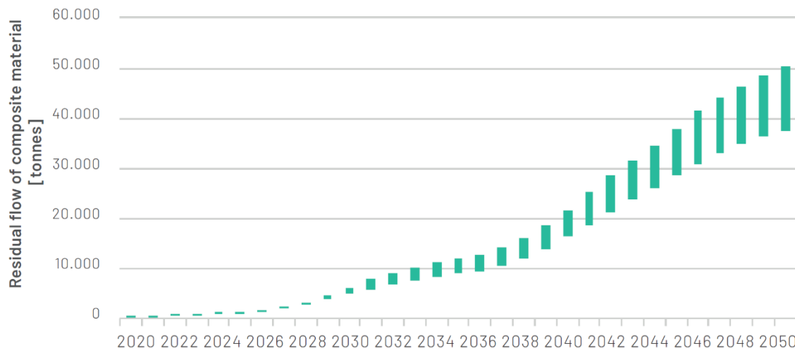
Figure 25: Residual flow of composite material [tonnes] resulting from offshore wind farm decommissioning in the southern North Sea (Hajonides et al., 2020).
