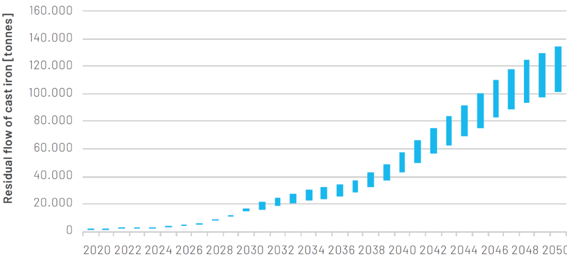
Figure 22: Residual flow of cast iron [tonnes] resulting from offshore wind farm decommissioning in the southern North Sea (Hajonides et al., 2020).
