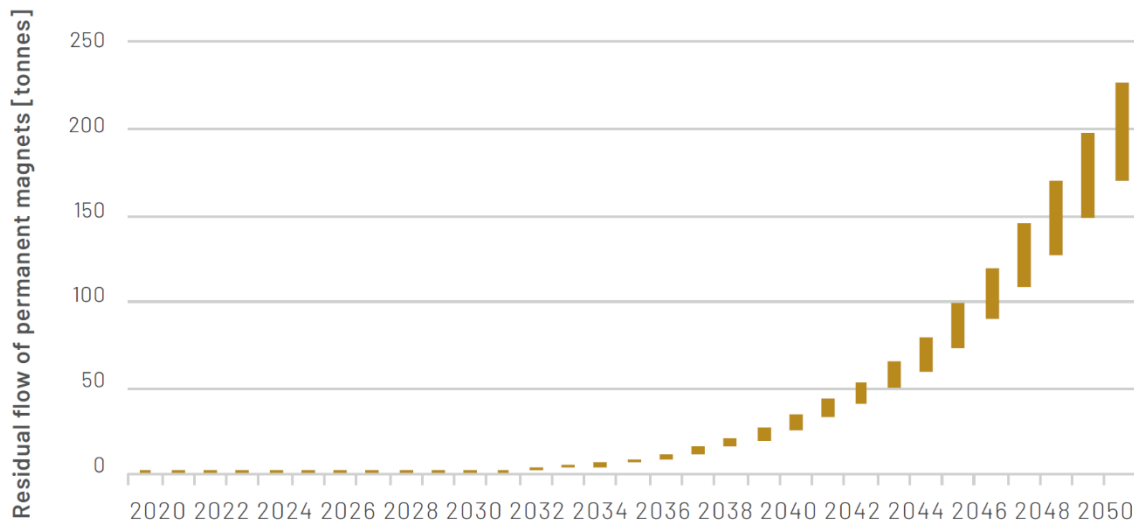
Figure 24: Residual flow of neodymium alloy permanent magnets [tonnes] (NdFeB) resulting from offshore wind farms decommissioning in the Southern North Sea (Hajonides et al., 2020).
